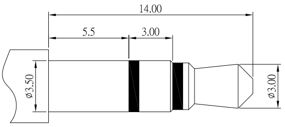
φ3.50mm 3 POLE PLUG
