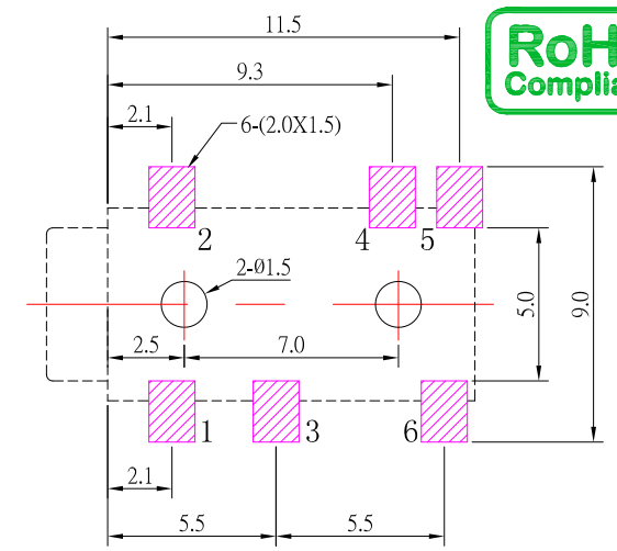
P.C.B LAYOUT TOP VIEW SCHEMATIC
